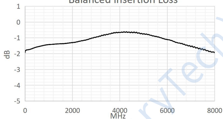
Balanced Insertion Loss
