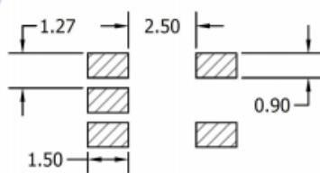
FOOTPRINT FOR PCB
